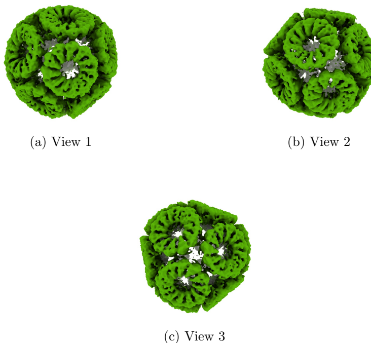
Figure 4: Isosurface at threshold=0.452000. Views generated by ChimeraX at a the following X, Y, Z angles: View 1 (0, -90, -90), View 2 (-90, 0, -90), View 3 (0, 0, 0).
