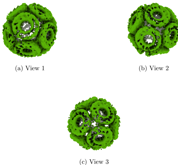
Figure 4: Isosurface at threshold=0.531000. Views generated by ChimeraX at a the following X, Y, Z angles: View 1 (0, -90, -90), View 2 (-90, 0, -90), View 3 (0, 0, 0).
