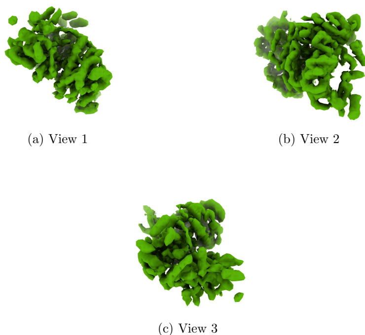
Figure 4: Isosurface at threshold=0.027200. Views generated by ChimeraX at a the following X, Y, Z angles: View 1 (0, -90, -90), View 2 (-90, 0, -90), View 3 (0, 0, 0).
