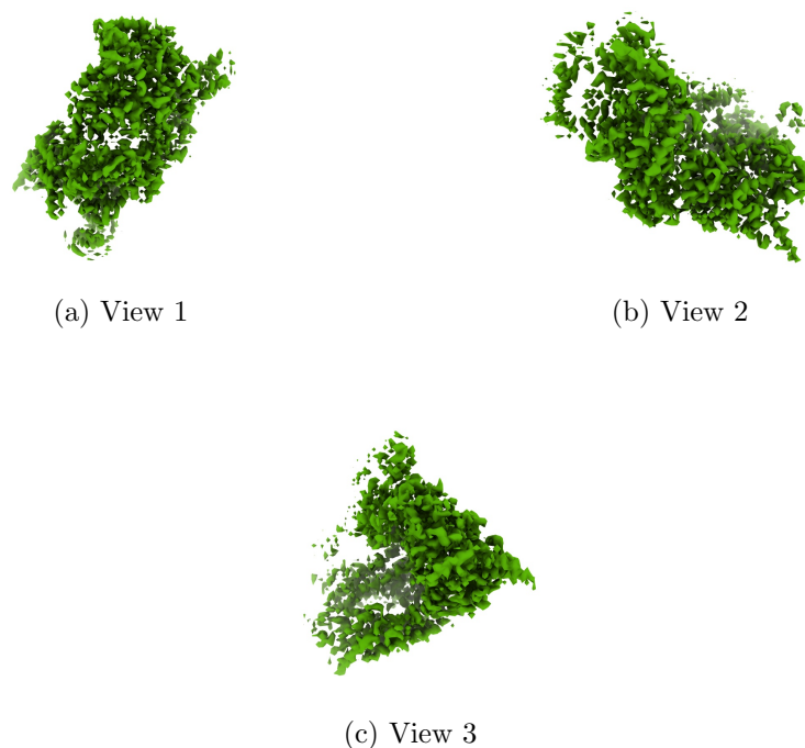
Figure 4: Isosurface at threshold=0.040700. Views generated by ChimeraX at a the following X, Y, Z angles: View 1 (0, -90, -90), View 2 (-90, 0, -90), View 3 (0, 0, 0).
