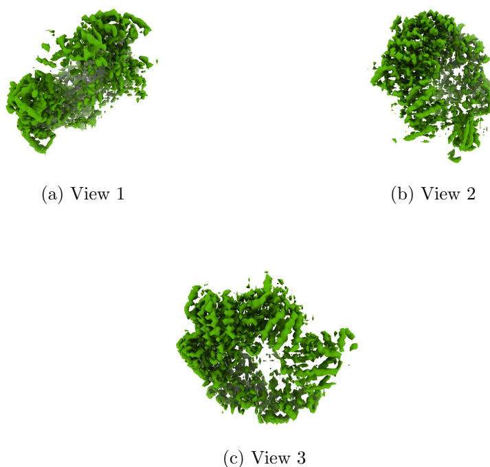
Figure 4: Isosurface at threshold=0.033300. Views generated by ChimeraX at a the following X, Y, Z angles: View 1 (0, -90, -90), View 2 (-90, 0, -90), View 3 (0, 0, 0).
