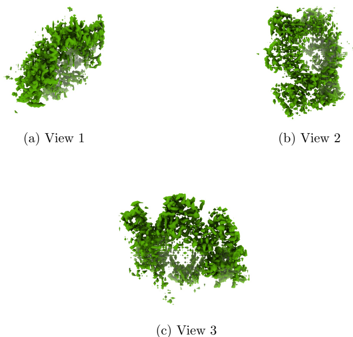
Figure 4: Isosurface at threshold=0.036900. Views generated by ChimeraX at a the following X, Y, Z angles: View 1 (0, -90, -90), View 2 (-90, 0, -90), View 3 (0, 0, 0).
