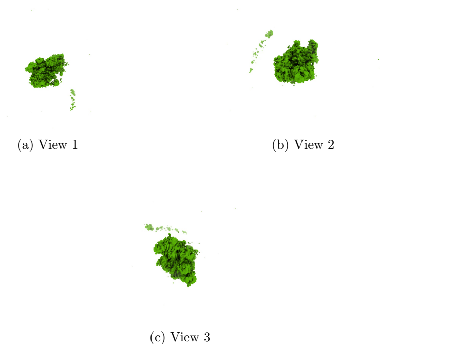
Figure 4: Isosurface at threshold=0.014400. Views generated by ChimeraX at a the following X, Y, Z angles: View 1 (0, -90, -90), View 2 (-90, 0, -90), View 3 (0, 0, 0).
