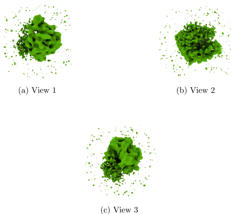
Figure 4: Isosurface at threshold=20.000000. Views generated by ChimeraX at a the following X, Y, Z angles: View 1 (0, -90, -90), View 2 (-90, 0, -90), View 3 (0, 0, 0).
