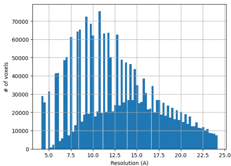
Figure 24: Histogram of the local resolution according to MonoRes.
