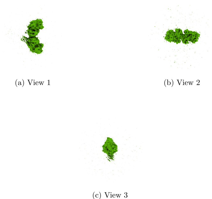
Figure 4: Isosurface at threshold=0.074300. Views generated by ChimeraX at a the following X, Y, Z angles: View 1 (0, -90, -90), View 2 (-90, 0, -90), View 3 (0, 0, 0).
