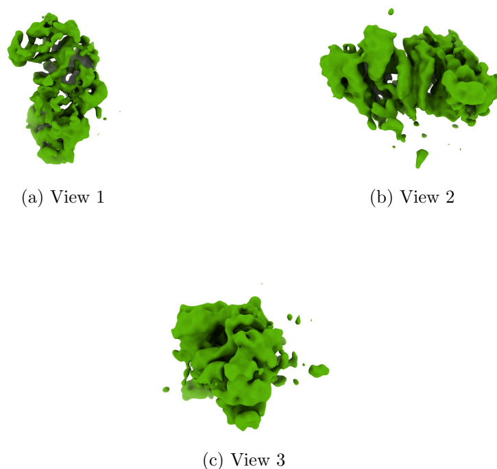
Figure 4: Isosurface at threshold=0.070100. Views generated by ChimeraX at a the following X, Y, Z angles: View 1 (0, -90, -90), View 2 (-90, 0, -90), View 3 (0, 0, 0).
