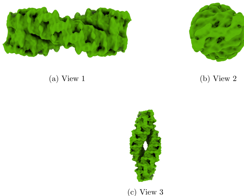
Figure 4: Isosurface at threshold=2.160000. Views generated by ChimeraX at a the following X, Y, Z angles: View 1 (0, -90, -90), View 2 (-90, 0, -90), View 3 (0, 0, 0).
