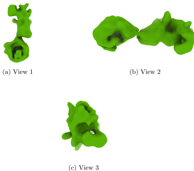
Figure 4: Isosurface at threshold=0.233000. Views generated by ChimeraX at a the following X, Y, Z angles: View 1 (0, -90, -90), View 2 (-90, 0, -90), View 3 (0, 0, 0).
