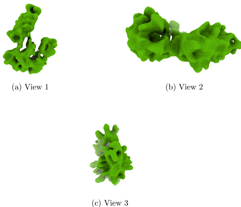
Figure 4: Isosurface at threshold=0.312000. Views generated by ChimeraX at a the following X, Y, Z angles: View 1 (0, -90, -90), View 2 (-90, 0, -90), View 3 (0, 0, 0).
