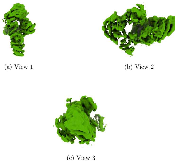
Figure 4: Isosurface at threshold=0.262000. Views generated by ChimeraX at a the following X, Y, Z angles: View 1 (0, -90, -90), View 2 (-90, 0, -90), View 3 (0, 0, 0).
