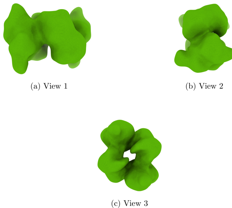
Figure 4: Isosurface at threshold=2.650000. Views generated by ChimeraX at a the following X, Y, Z angles: View 1 (0, -90, -90), View 2 (-90, 0, -90), View 3 (0, 0, 0).
