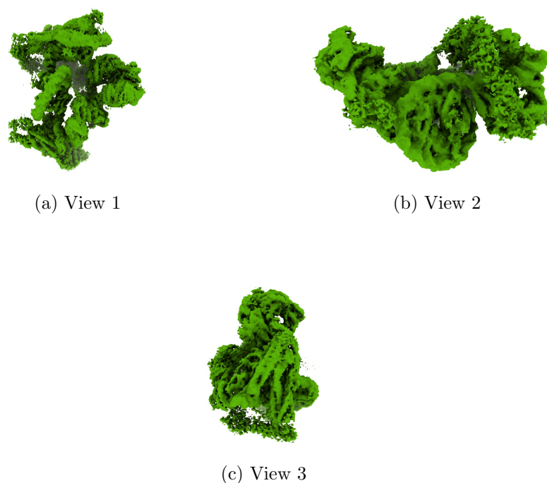
Figure 4: Isosurface at threshold=0.004610. Views generated by ChimeraX at a the following X, Y, Z angles: View 1 (0, -90, -90), View 2 (-90, 0, -90), View 3 (0, 0, 0).
