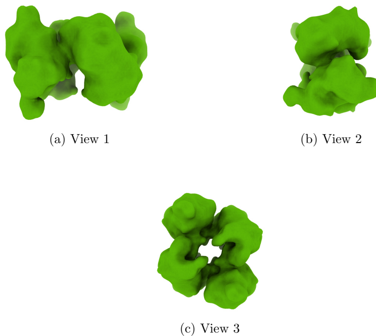
Figure 4: Isosurface at threshold=3.440000. Views generated by ChimeraX at a the following X, Y, Z angles: View 1 (0, -90, -90), View 2 (-90, 0, -90), View 3 (0, 0, 0).
