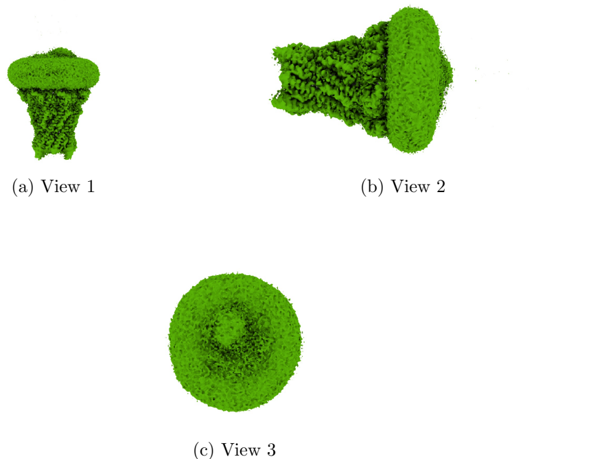
Figure 4: Isosurface at threshold=0.035000. Views generated by ChimeraX at a the following X, Y, Z angles: View 1 (0, -90, -90), View 2 (-90, 0, -90), View 3 (0, 0, 0).
