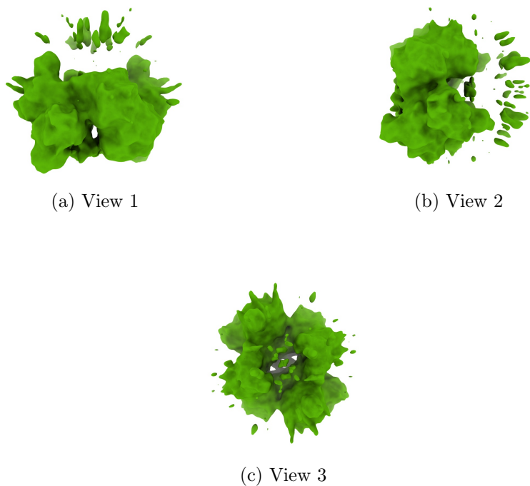
Figure 4: Isosurface at threshold=2.550000. Views generated by ChimeraX at a the following X, Y, Z angles: View 1 (0, -90, -90), View 2 (-90, 0, -90), View 3 (0, 0, 0).
