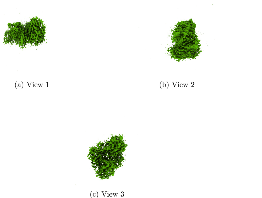
Figure 4: Isosurface at threshold=0.013000. Views generated by ChimeraX at a the following X, Y, Z angles: View 1 (0, -90, -90), View 2 (-90, 0, -90), View 3 (0, 0, 0).
