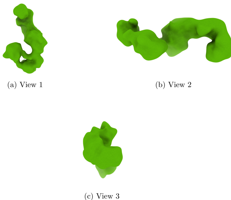
Figure 4: Isosurface at threshold=1.900000. Views generated by ChimeraX at a the following X, Y, Z angles: View 1 (0, -90, -90), View 2 (-90, 0, -90), View 3 (0, 0, 0).
