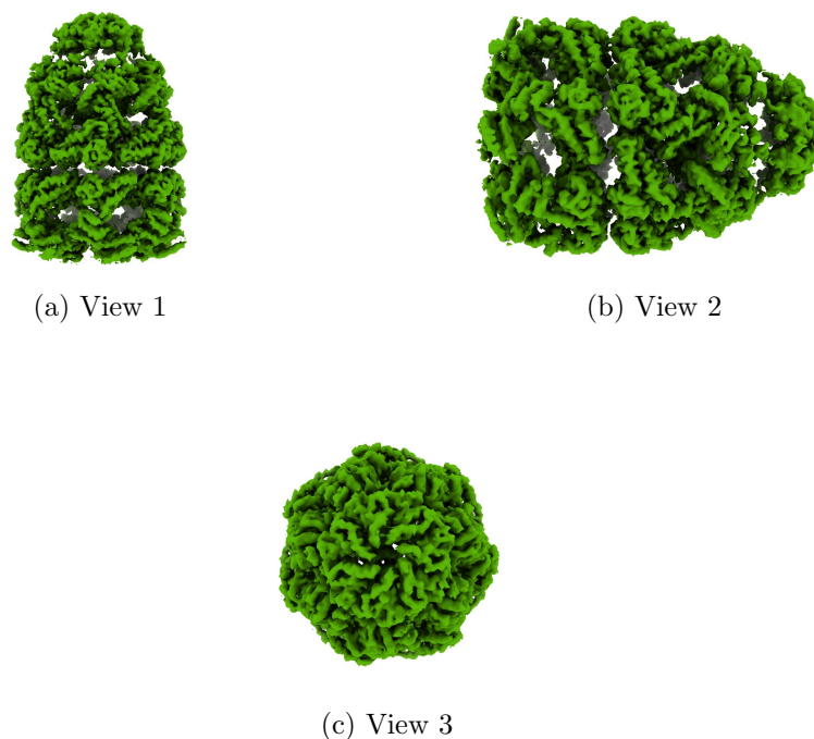
Figure 4: Isosurface at threshold=0.369000. Views generated by ChimeraX at a the following X, Y, Z angles: View 1 (0, -90, -90), View 2 (-90, 0, -90), View 3 (0, 0, 0).
