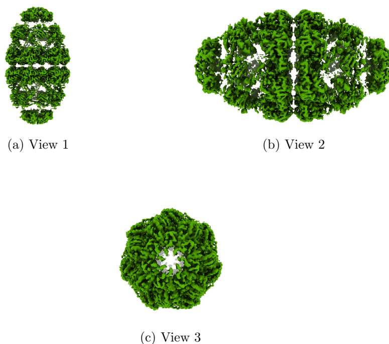
Figure 4: Isosurface at threshold=0.529000. Views generated by ChimeraX at a the following X, Y, Z angles: View 1 (0, -90, -90), View 2 (-90, 0, -90), View 3 (0, 0, 0).
