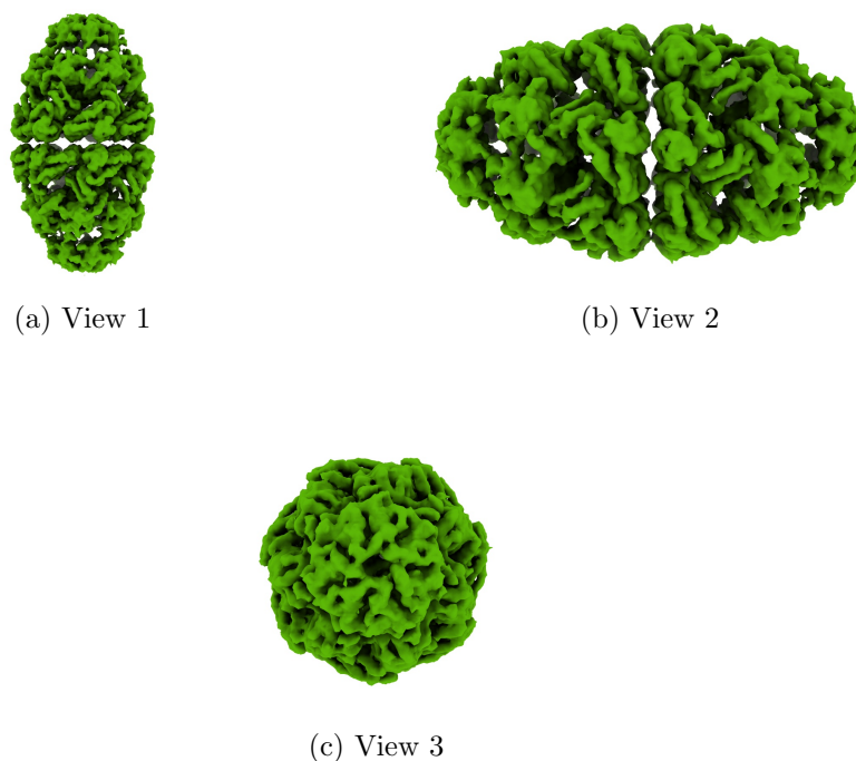
Figure 4: Isosurface at threshold=0.267000. Views generated by ChimeraX at a the following X, Y, Z angles: View 1 (0, -90, -90), View 2 (-90, 0, -90), View 3 (0, 0, 0).
