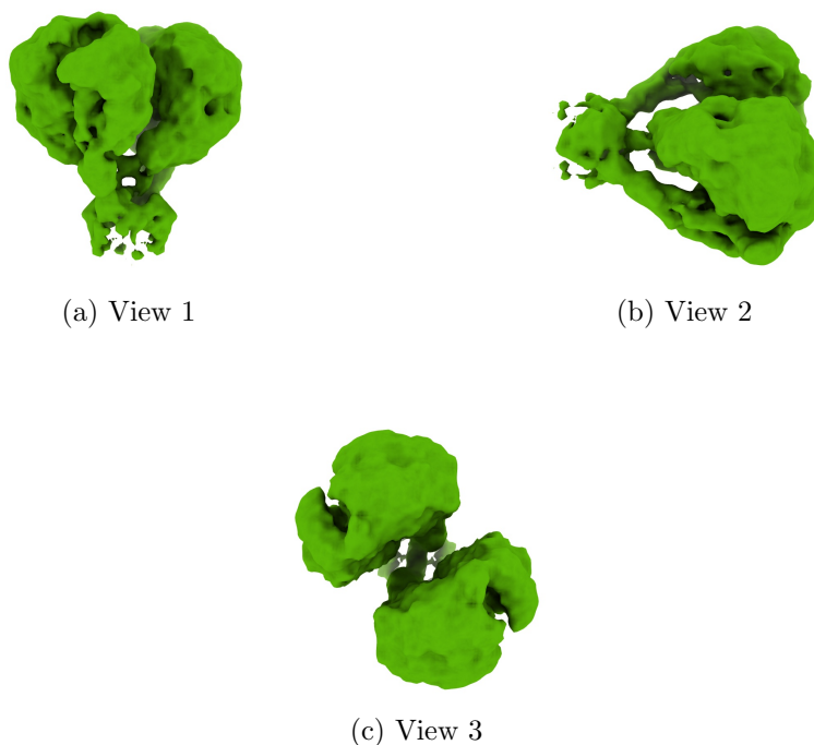
Figure 4: Isosurface at threshold=0.053100. Views generated by ChimeraX at a the following X, Y, Z angles: View 1 (0, -90, -90), View 2 (-90, 0, -90), View 3 (0, 0, 0).
