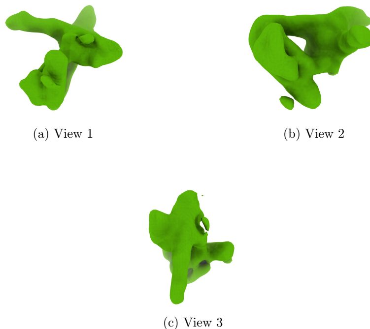
Figure 4: Isosurface at threshold=0.002380. Views generated by ChimeraX at a the following X, Y, Z angles: View 1 (0, -90, -90), View 2 (-90, 0, -90), View 3 (0, 0, 0).
