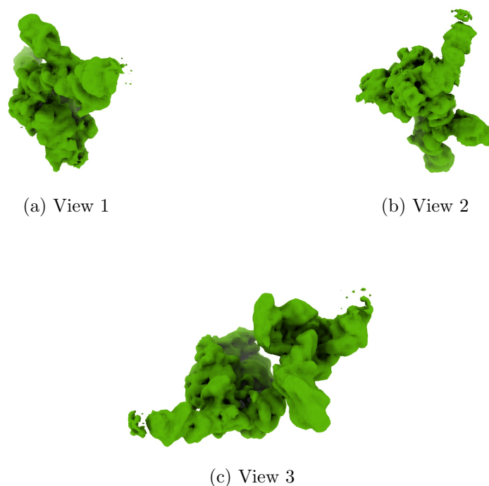
Figure 4: Isosurface at threshold=0.006000. Views generated by ChimeraX at a the following X, Y, Z angles: View 1 (0, -90, -90), View 2 (-90, 0, -90), View 3 (0, 0, 0).
