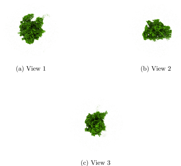
Figure 4: Isosurface at threshold=0.765000. Views generated by ChimeraX at a the following X, Y, Z angles: View 1 (0, -90, -90), View 2 (-90, 0, -90), View 3 (0, 0, 0).
