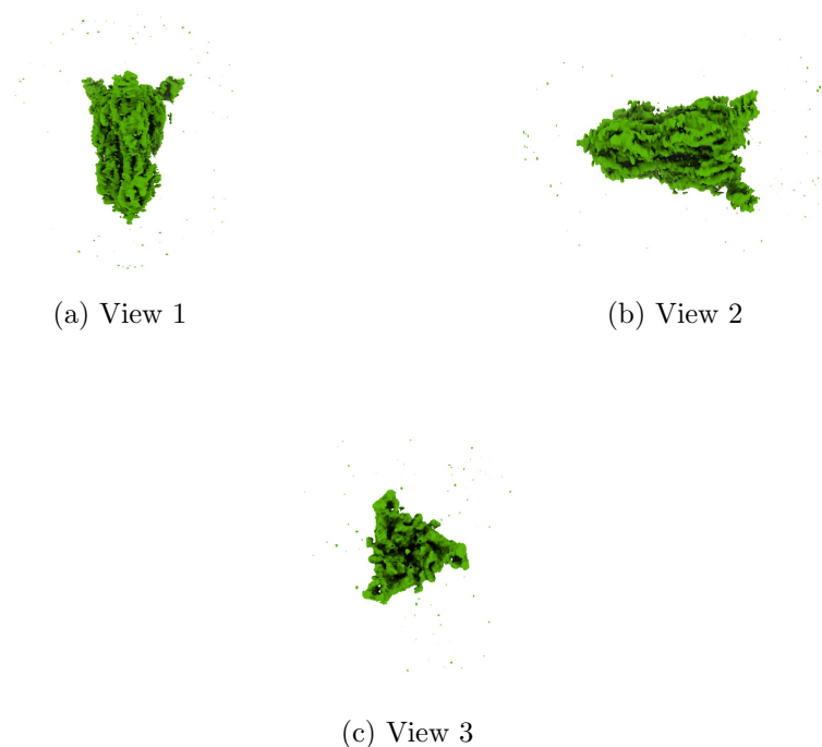
Figure 4: Isosurface at threshold=0.010600. Views generated by ChimeraX at a the following X, Y, Z angles: View 1 (0, -90, -90), View 2 (-90, 0, -90), View 3 (0, 0, 0).
