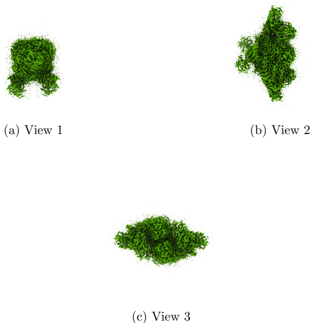
Figure 4: Isosurface at threshold=0.040000. Views generated by ChimeraX at a the following X, Y, Z angles: View 1 (0, -90, -90), View 2 (-90, 0, -90), View 3 (0, 0, 0).
