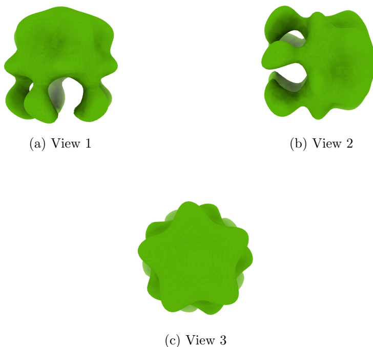
Figure 4: Isosurface at threshold=0.022500. Views generated by ChimeraX at a the following X, Y, Z angles: View 1 (0, -90, -90), View 2 (-90, 0, -90), View 3 (0, 0, 0).
