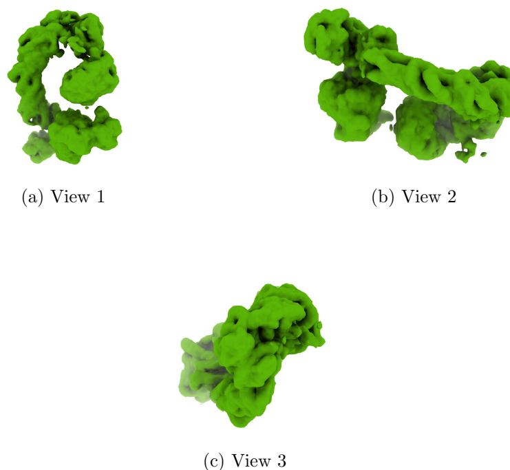
Figure 4: Isosurface at threshold=0.024400. Views generated by ChimeraX at a the following X, Y, Z angles: View 1 (0, -90, -90), View 2 (-90, 0, -90), View 3 (0, 0, 0).
