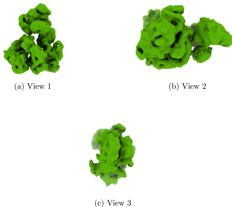
Figure 4: Isosurface at threshold=0.251000. Views generated by ChimeraX at a the following X, Y, Z angles: View 1 (0, -90, -90), View 2 (-90, 0, -90), View 3 (0, 0, 0).
