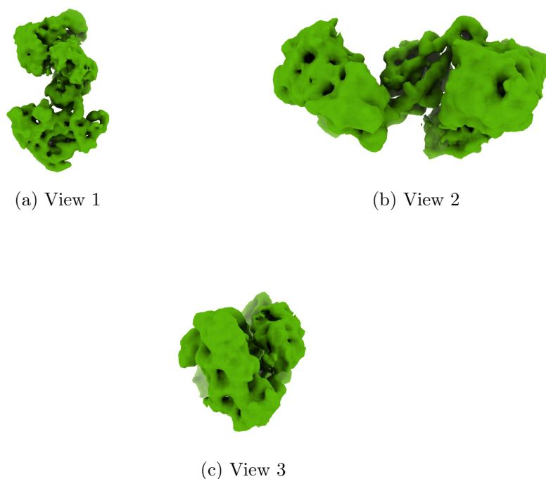
Figure 4: Isosurface at threshold=0.371000. Views generated by ChimeraX at a the following X, Y, Z angles: View 1 (0, -90, -90), View 2 (-90, 0, -90), View 3 (0, 0, 0).
