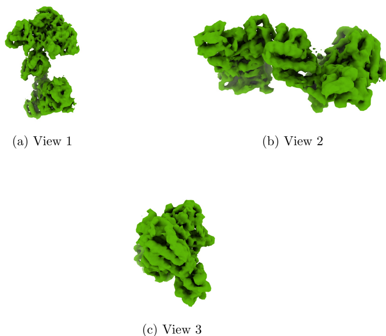
Figure 4: Isosurface at threshold=0.217000. Views generated by ChimeraX at a the following X, Y, Z angles: View 1 (0, -90, -90), View 2 (-90, 0, -90), View 3 (0, 0, 0).
