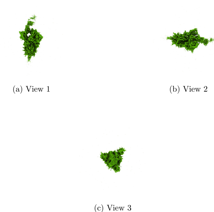
Figure 4: Isosurface at threshold=0.145000. Views generated by ChimeraX at a the following X, Y, Z angles: View 1 (0, -90, -90), View 2 (-90, 0, -90), View 3 (0, 0, 0).
