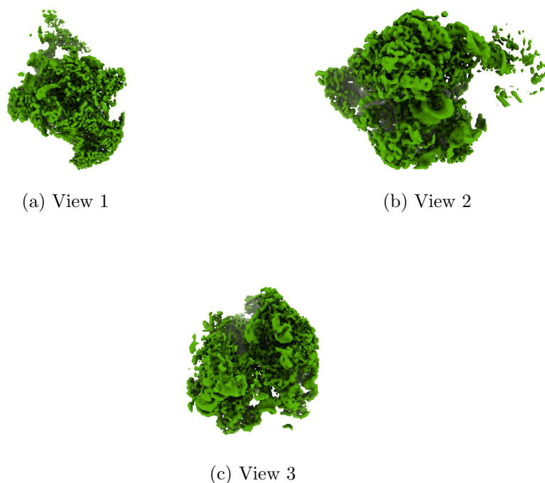
Figure 4: Isosurface at threshold=0.750000. Views generated by ChimeraX at a the following X, Y, Z angles: View 1 (0, -90, -90), View 2 (-90, 0, -90), View 3 (0, 0, 0).
