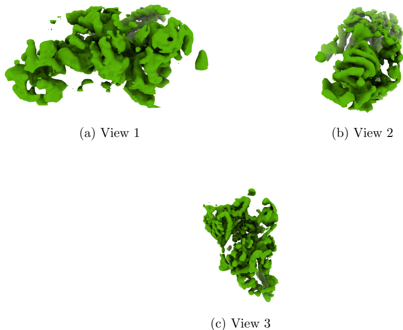
Figure 4: Isosurface at threshold=0.500000. Views generated by ChimeraX at a the following X, Y, Z angles: View 1 (0, -90, -90), View 2 (-90, 0, -90), View 3 (0, 0, 0).
