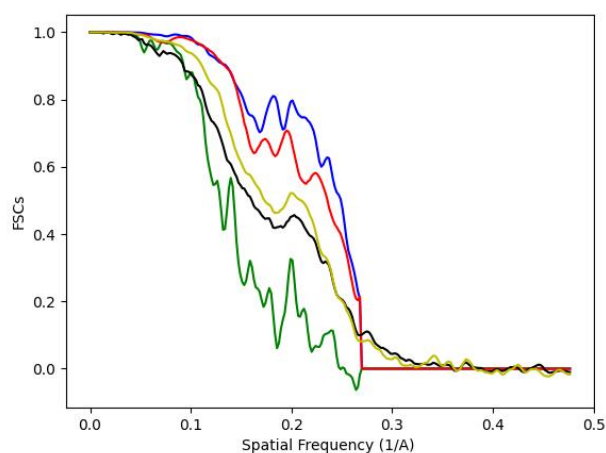
Figure 33: FSC in X, Y, Z, the global FSC, and the Average Cosine Phase.
