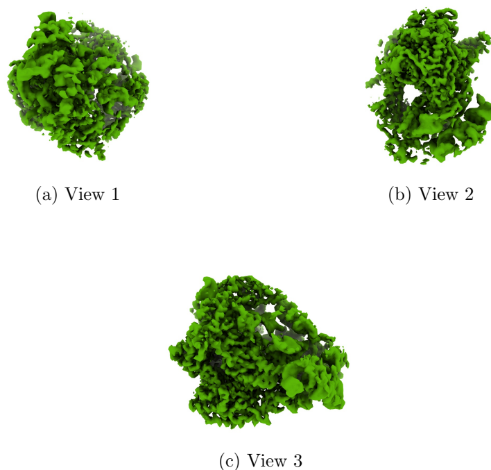
Figure 4: Isosurface at threshold=0.650000. Views generated by ChimeraX at the following X, Y, Z angles: View 1 (0, -90, -90), View 2 (-90, 0, -90), View 3 (0, 0, 0).
