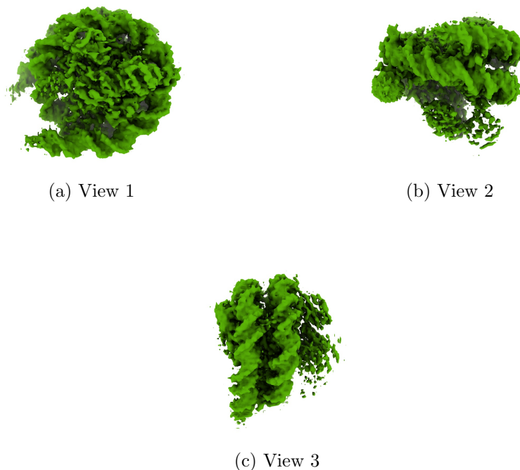
Figure 4: Isosurface at threshold=0.263000. Views generated by ChimeraX at a the following X, Y, Z angles: View 1 (0, -90, -90), View 2 (-90, 0, -90), View 3 (0, 0, 0).
