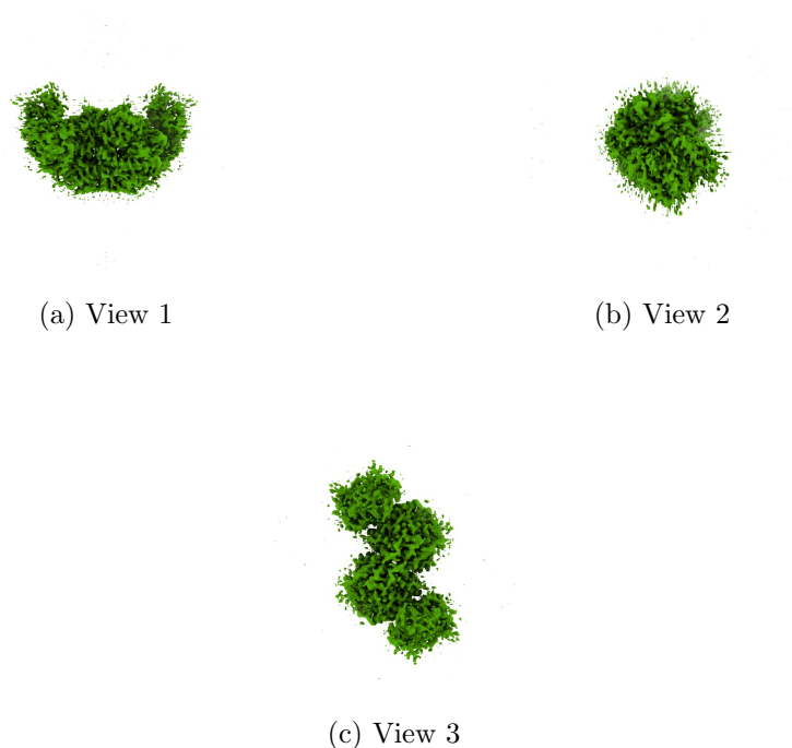
Figure 4: Isosurface at threshold=0.272000. Views generated by ChimeraX at a the following X, Y, Z angles: View 1 (0, -90, -90), View 2 (-90, 0, -90), View 3 (0, 0, 0).
