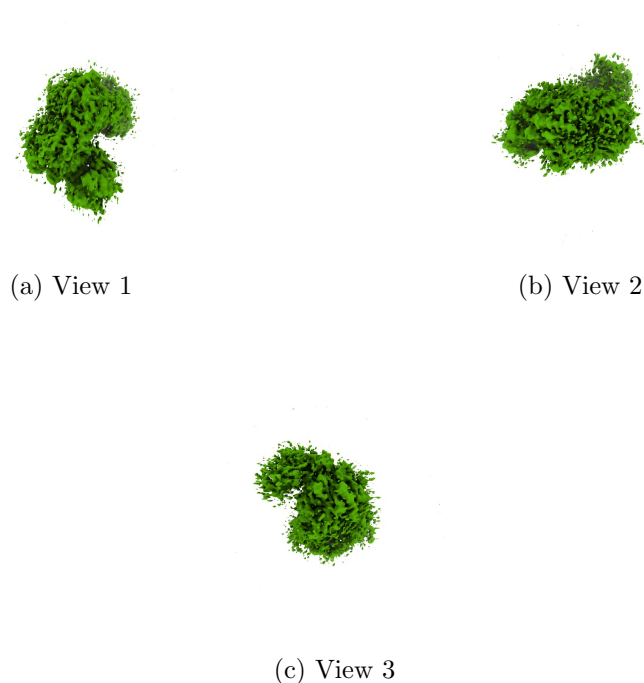
Figure 4: Isosurface at threshold=0.216000. Views generated by ChimeraX at a the following X, Y, Z angles: View 1 (0, -90, -90), View 2 (-90, 0, -90), View 3 (0, 0, 0).
