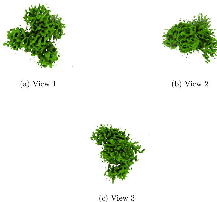
Figure 4: Isosurface at threshold=0.255000. Views generated by ChimeraX at a the following X, Y, Z angles: View 1 (0, -90, -90), View 2 (-90, 0, -90), View 3 (0, 0, 0).
