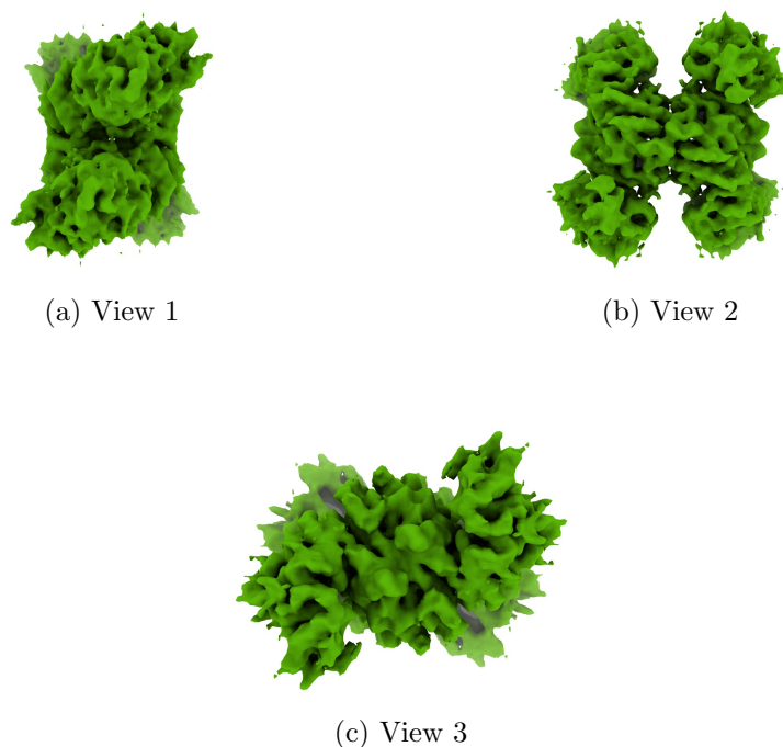
Figure 4: Isosurface at threshold=0.143000. Views generated by ChimeraX at a the following X, Y, Z angles: View 1 (0, -90, -90), View 2 (-90, 0, -90), View 3 (0, 0, 0).
