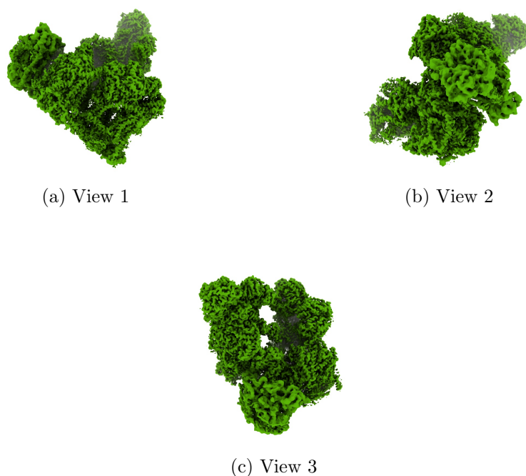
Figure 4: Isosurface at threshold=0.015000. Views generated by ChimeraX at the following X, Y, Z angles: View 1 (0, -90, -90), View 2 (-90, 0, -90), View 3 (0, 0, 0).
