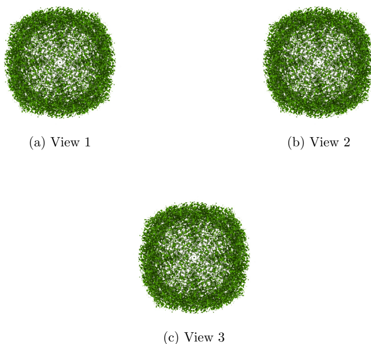
Figure 4: Isosurface at threshold=0.038200. Views generated by ChimeraX at a the following X, Y, Z angles: View 1 (0, -90, -90), View 2 (-90, 0, -90), View 3 (0, 0, 0).
