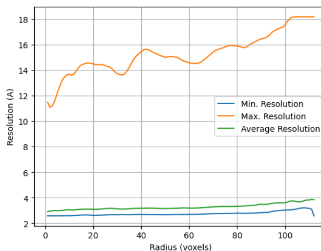
Figure 26: Radial averages (in space) of the minimum, maximum and average resolution at each voxel.
