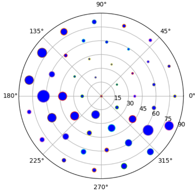
Figure 25: Histogram 2D of the best direction at each voxel. The azimuthal rotation is circular, while the tilt angle is the radius. The size of the point is proportional to the number of voxels whose maximum resolution is in that direction (this count can be seen in Fig. 24).
