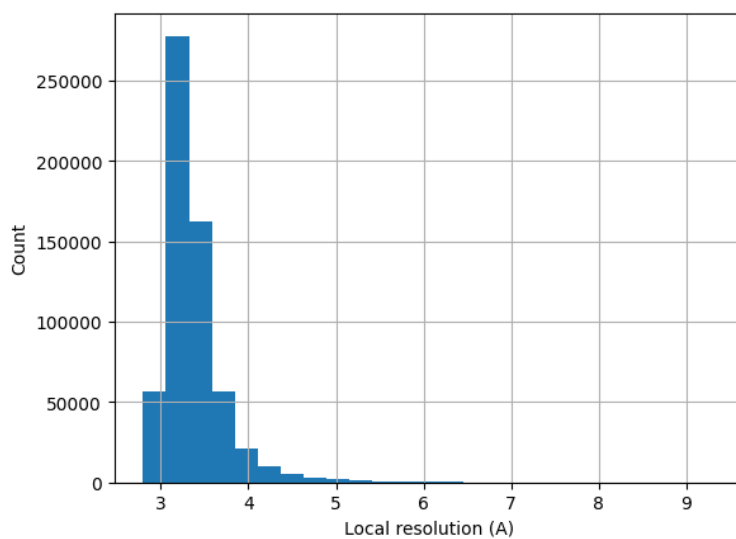
Figure 22: Histogram of the local resolution according to blocres.
