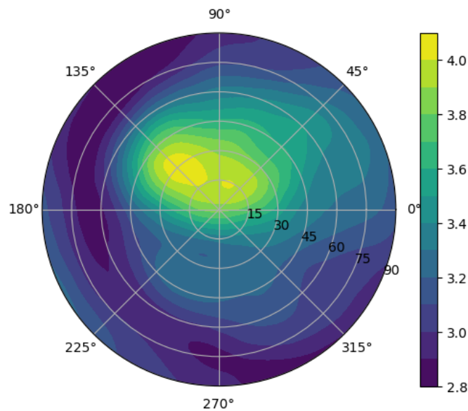
Figure 30: Directional resolution in the projection sphere.
