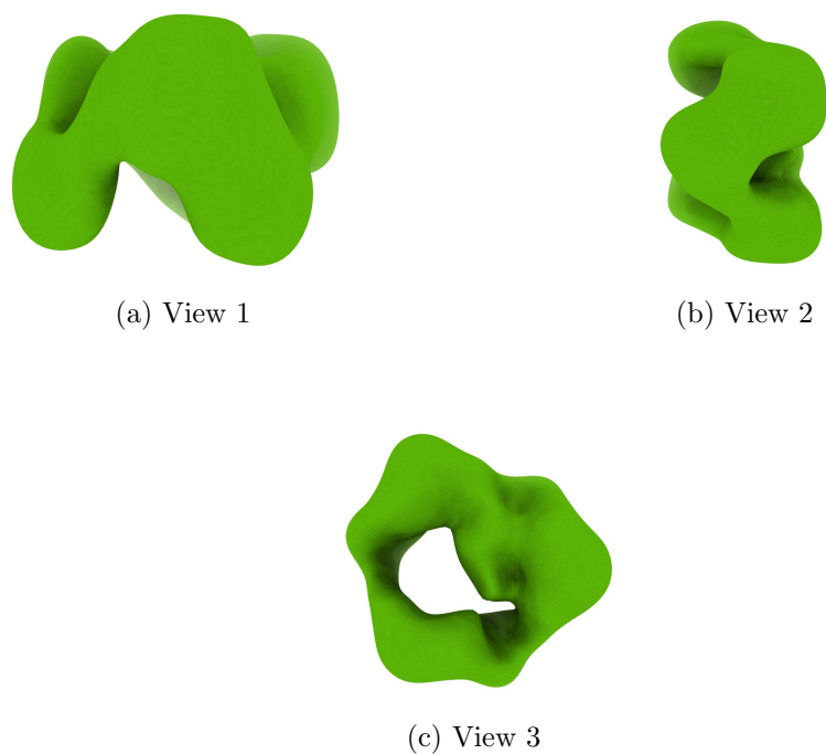
Figure 4: Isosurface at threshold=0.268000. Views generated by ChimeraX at a the following X, Y, Z angles: View 1 (0, -90, -90), View 2 (-90, 0, -90), View 3 (0, 0, 0).
